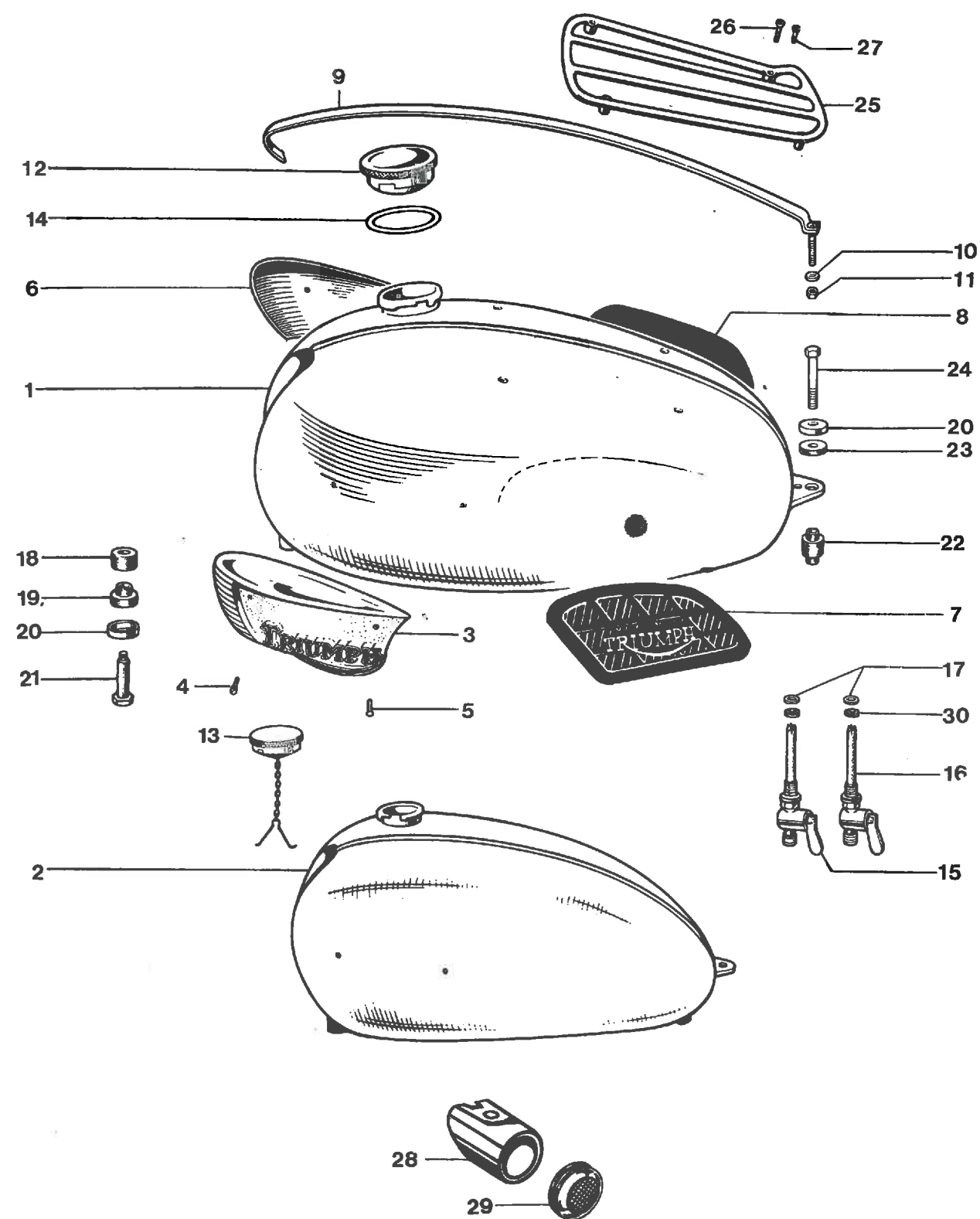
Fig. 22. GAS TANKS
