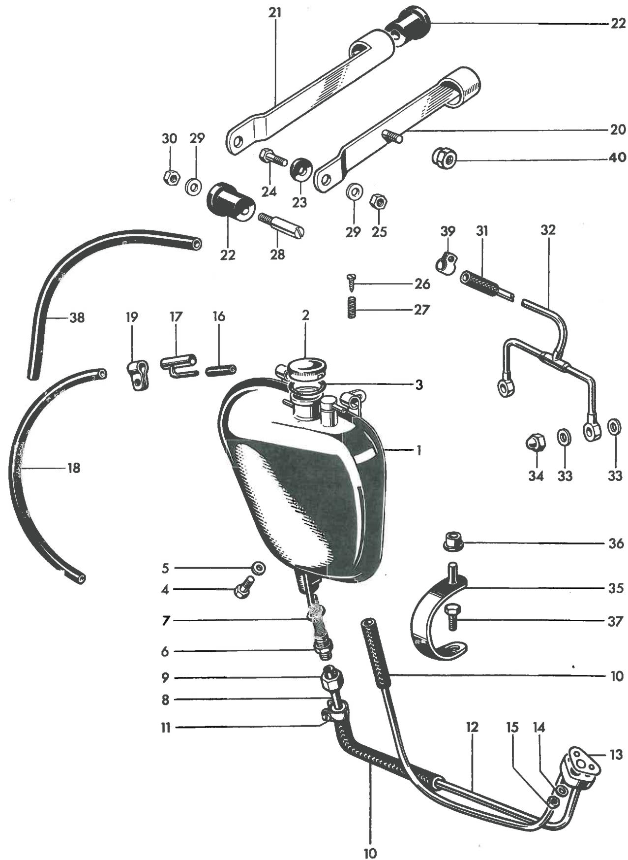
Fig. 23. OIL TANK 54
