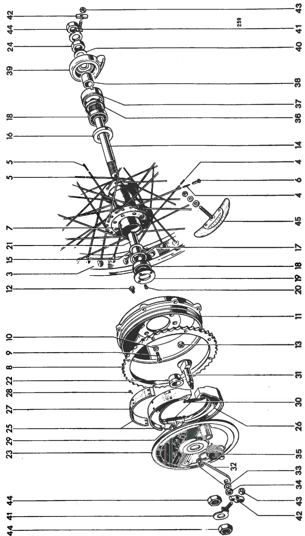
Fig. 20. REAR WHEEL
