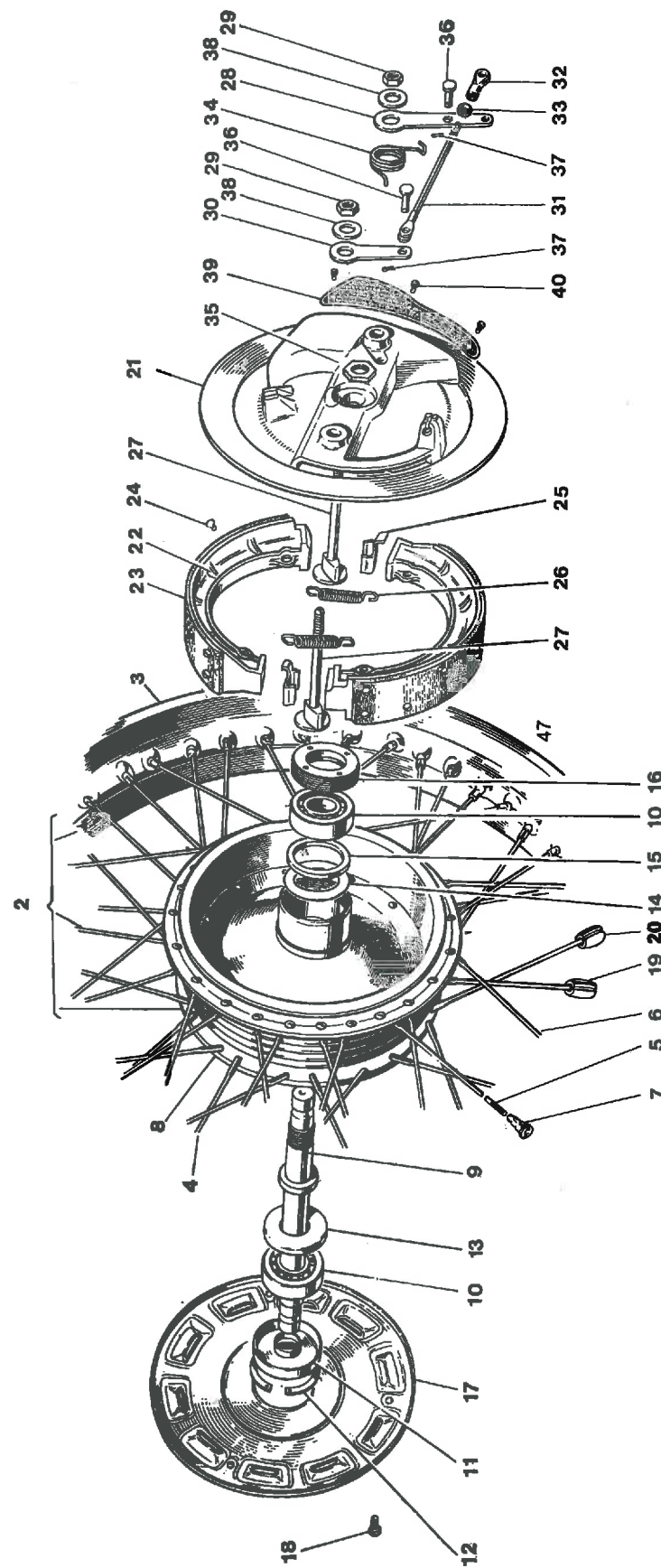
Fig. 19. FRONT WHEEL
