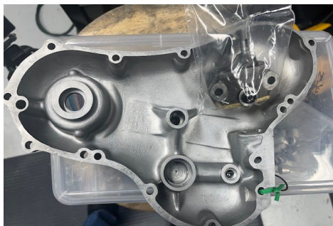
AMR Mods to timing cover for anti-wet sumping
