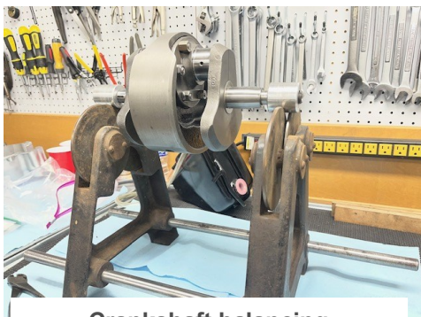
Crankshaft balancing
